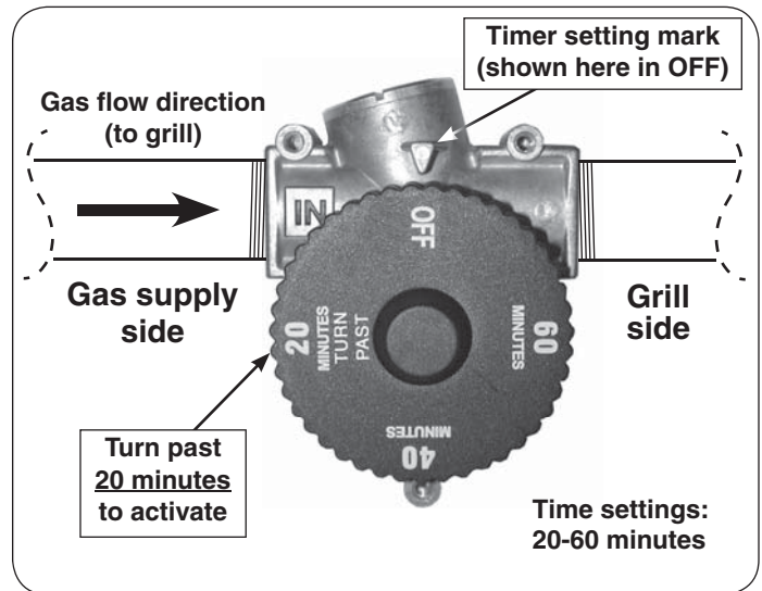
Fig. 1-1 Horizontal setup
