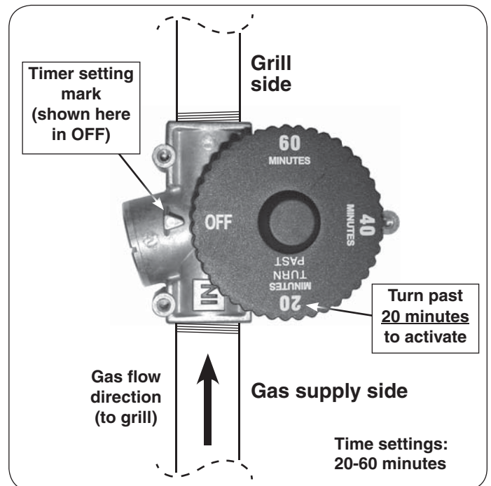
Fig. 1-2 Vertical setup
